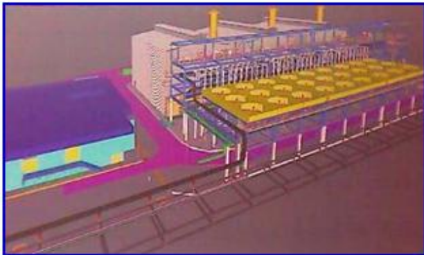
Weight Structure for On Shore Compressor
