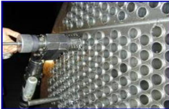
Fabrication of Stainless Steel Heat Exchanger
